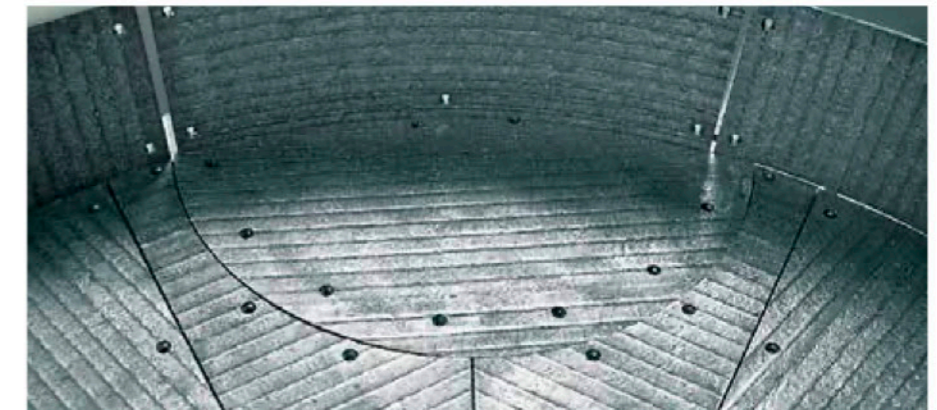
Lining of a mixer: the sidewalls, the bottom and the discharge elements have been protected with KALMETALL W100; diameter 3.500 mm.
