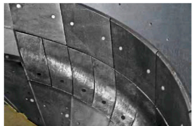
Screens are used in many areas of raw material processing. The herringbone pattern is burned in the KALMETALL hard overlay welded plates.
