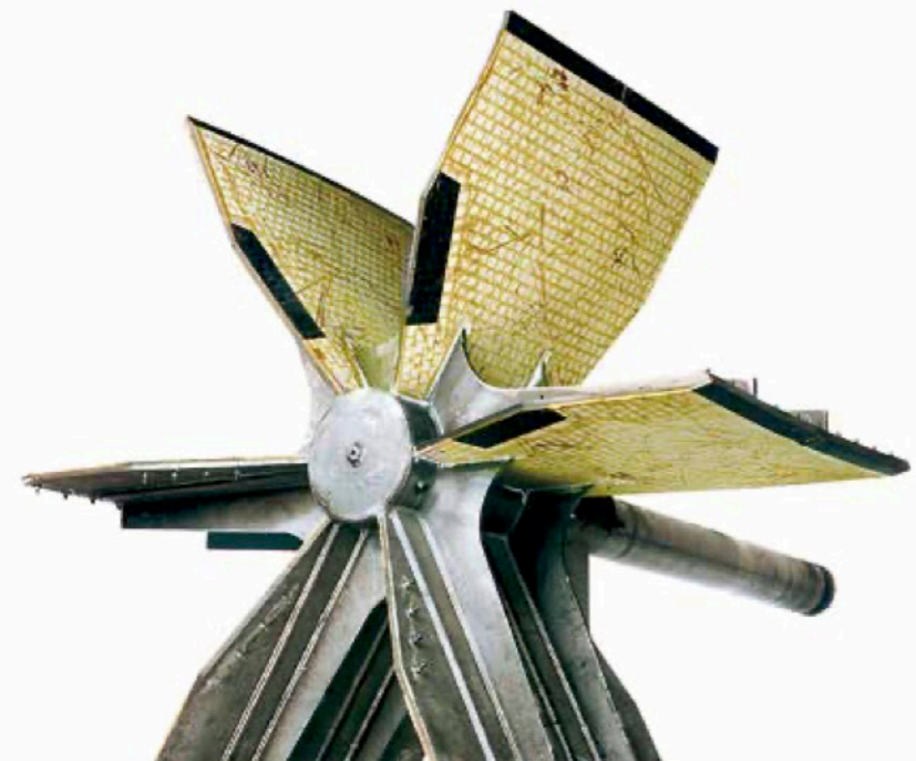
In case of extreme wear, the fan blades can be protected by KALOCER high alumina ceramics. Due to the high rotational speed a high performance adhesive is used.
